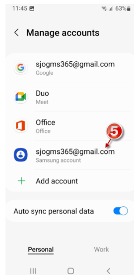
Figure 5: Email List
