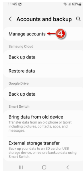
Figure 4: Manage Accounts
