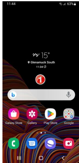
Figure 1: Phone Screen
