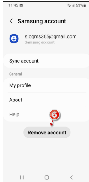
Figure 6: Remove Account
