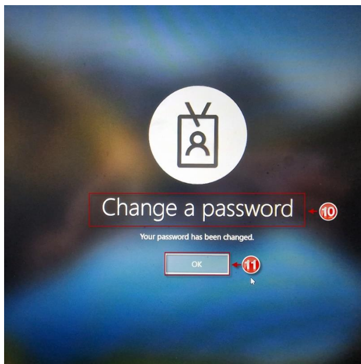
Figure 7: Password Changed
