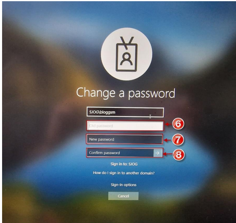
Figure 5: Changing Password.
