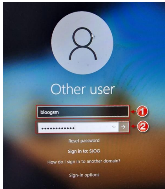
Figure 1: Login Screen
