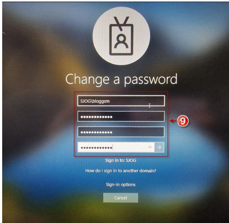
Figure 6: Changed Password
