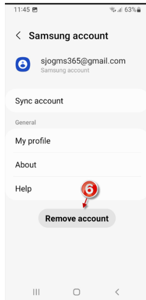
Figure 6: Remove Account
