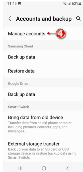
Figure 4: Manage Accounts
