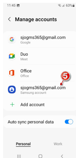
Figure 5: Email List
